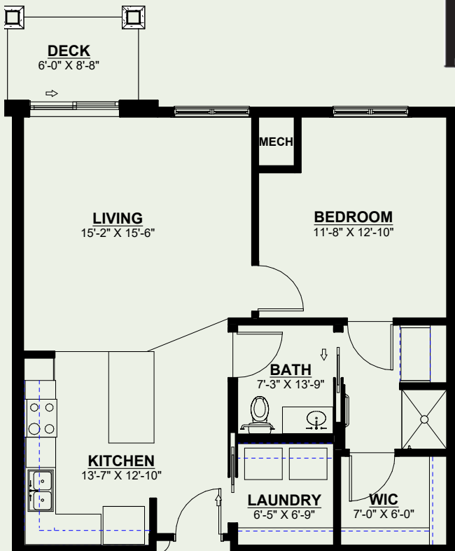
Pine 846 Sq. Ft. One Bedroom
