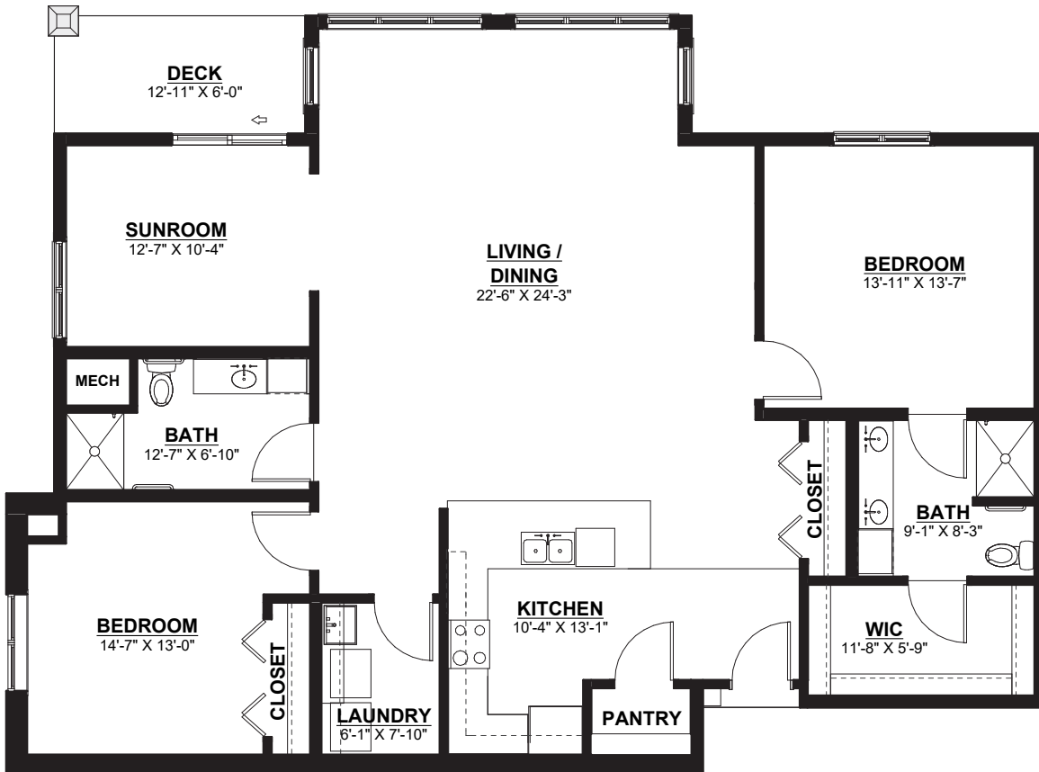
Basswood 1,752 Sq. Ft. Two Bedroom Plus/ Sunroom
